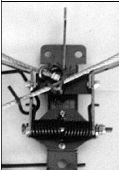
8. Mount the cable, utilizing the clips on the cable arms, ensuring the cable passes through the groove in the throw arm and under the hook of the cinch spring.
